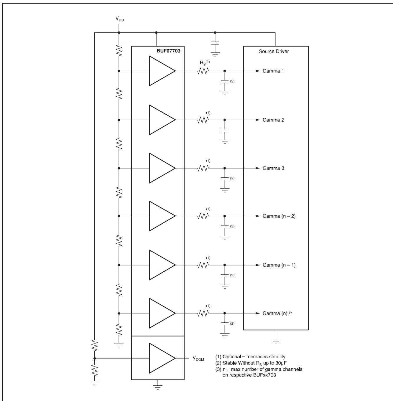
Figure 35. LCD Source Driver Typical Block Diagram.
